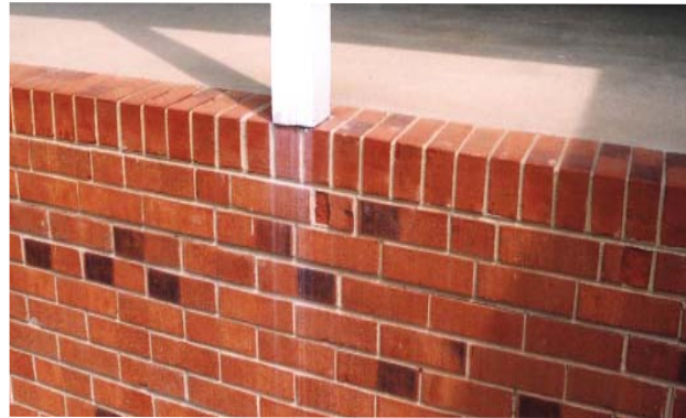
Photo 13 Runoff Stain from Paint
