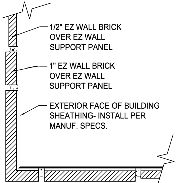
CORNER PLAN
