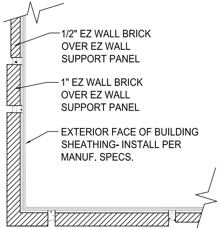
CORNER PLAN
